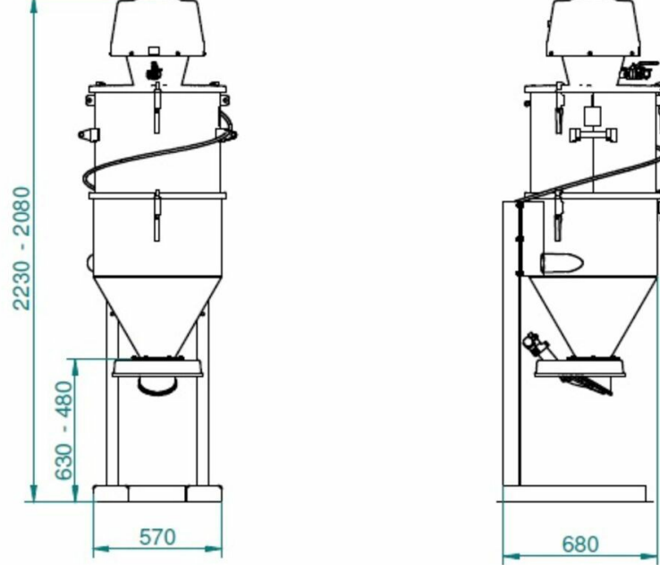
Dimensions - Filter part
